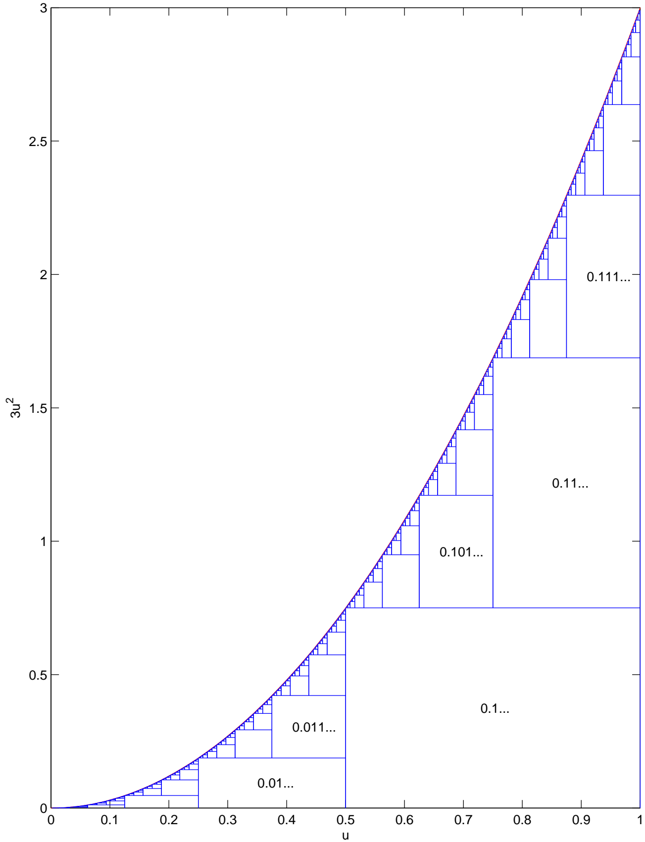
Exact binary sampling of power distribution
